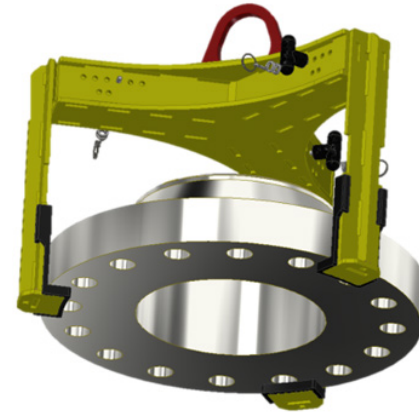
NPS 10, Class 600, Weld Neck Flange
