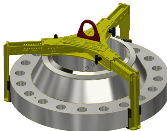
NPS 20, Class 900, Weld Neck Flange
